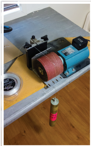
Prototype leaders and line are batch tested for abrasion resistance
