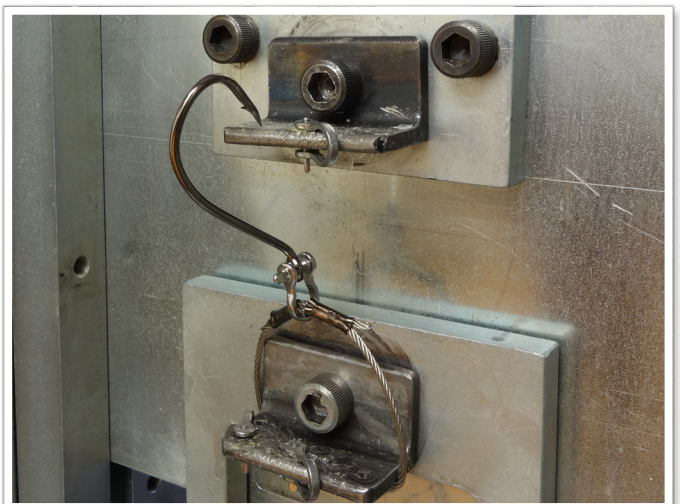
The "point loading" hook test
